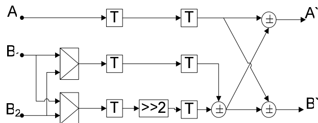
Figure 6 – Samples mixing – 8x8 transform only
