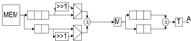
Figure 4 – Structure of computational block of 1-D 4-point inverse integer transform
