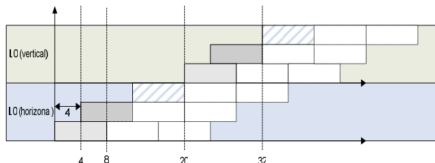
Figure 7 – Timing diagram
