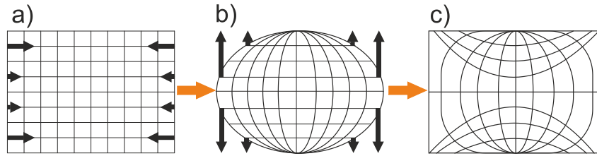
Figure 41: Fast reprojection of an equirectangular image (a) to transverse equirectangular image (c). Black arrows show direction of change of size of respective rows and columns of images
