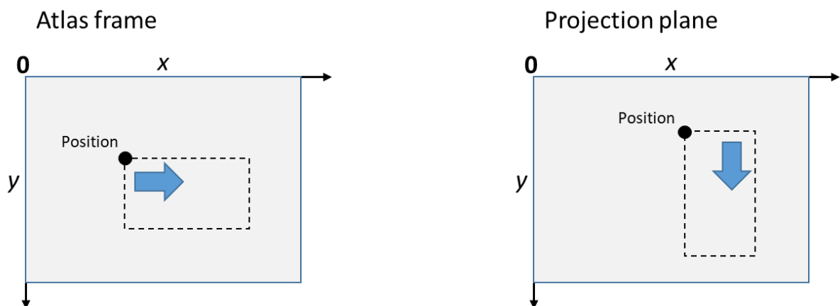
Figure 19: Definition of 90° patch rotation
