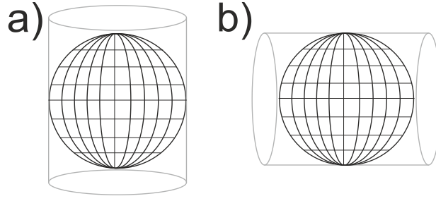
Figure 40: Cylinders used in the projection of a sphere on a flat image in a) equirectangular projection and b) transverse equirectangular projection
