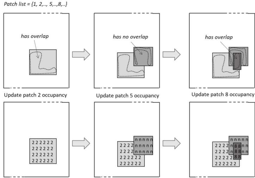
Figure 36. Occupancy map update in an ordered manner with patch culling
