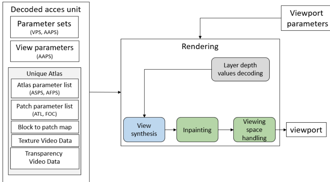
Figure 43: Process flow for TMIV MPI renderer
