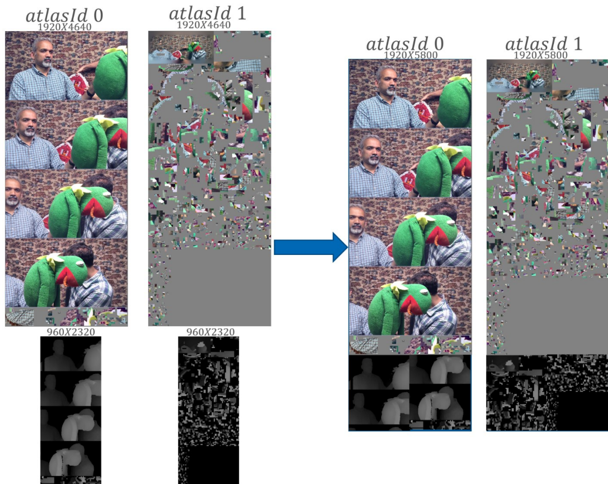
Figure 26: Frame packing for MIV anchor – Frog sequence at frame 0, featuring 3 regions
