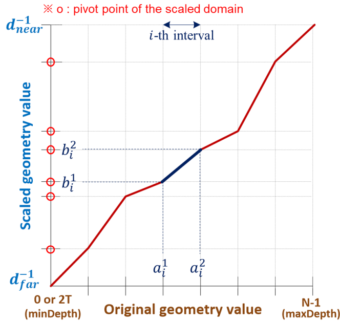
Figure 25: An example of piecewise linear scaling (for 7 intervals)
