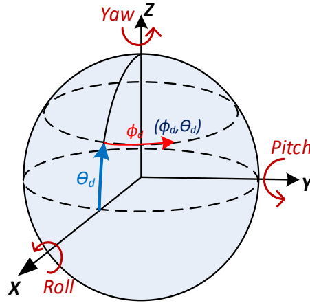
Figure 44: OMAF coordinate system illustrating the directions of positional and rotational units
