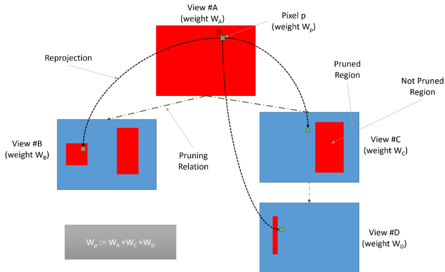
Figure 39: graph-based pruning: weight recovery procedure
