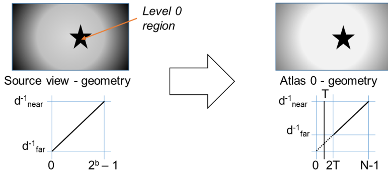
Figure 24: When the source material (with b bits per sample) has invalid geometry values, the geometry coder not only performs u(b) to u(m) or u(m - 1) scaling, but it also sets the geometry threshold to a configured value ( T ) and the normalized disparity range is modified such that value 2T corresponds to the far geometry; N = 2^m if the geometry has a good quality (§4.2.5) and 2^{m-1} otherwise
