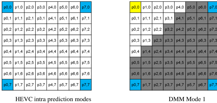
Figure 26: Selection of samples for calculating the predicted depth value in SDC (Planar mode, DMM Mode 1)
