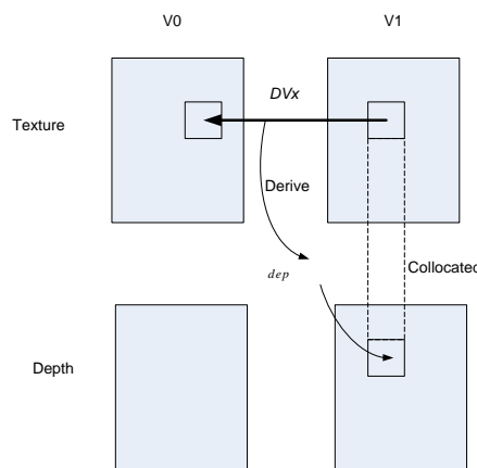
Figure 28: A depth value derived from its corresponding disparity vector
