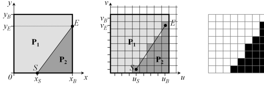
Figure 20: Wedgelet partition of a block: continuous (left) and discrete signal space (middle) with corresponding partition pattern (right).
