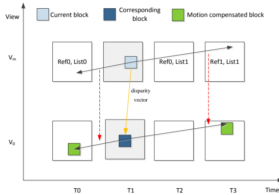
Figure 13: Relationship among current block, reference block and motion compensated block
