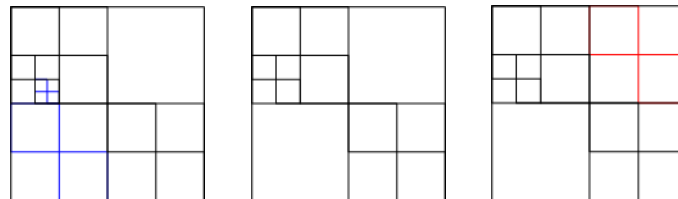
Figure 33: Example of a CTB QT partitioning for the texture (left), allowed collocated depth CTB QT partitioning (centre), and disallowed collocated depth CTB QT partitioning (right).
