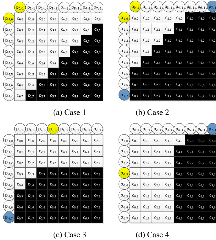
Figure 23: Selection of reference samples for difference partition pattern cases.
