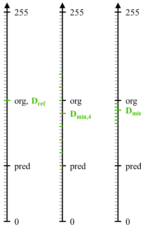
Figure 25: Optimized search strategy for non-quantized partition offset values.
