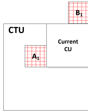
Figure 7: Example: For the derivation of the disparity from DV-MCP neighbouring blocks of the current CU, above block B1 is not used, since it is not located within the current CTU.
