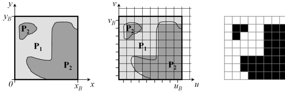
Figure 21: Contour partition of a block: continuous (left) and discrete signal space (middle) with corresponding partition pattern (right).
