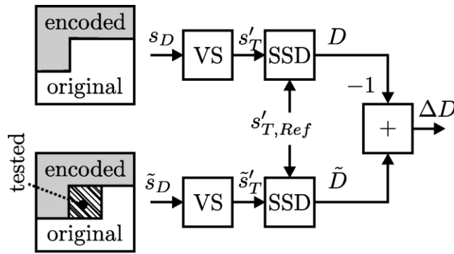
Figure 31: Definition of the SVDC related to the distorted depth data of the block B depicted by the hatched area in the bottom branch; VS denotes the view synthesis step and SSD stands for sum of squared differences.
