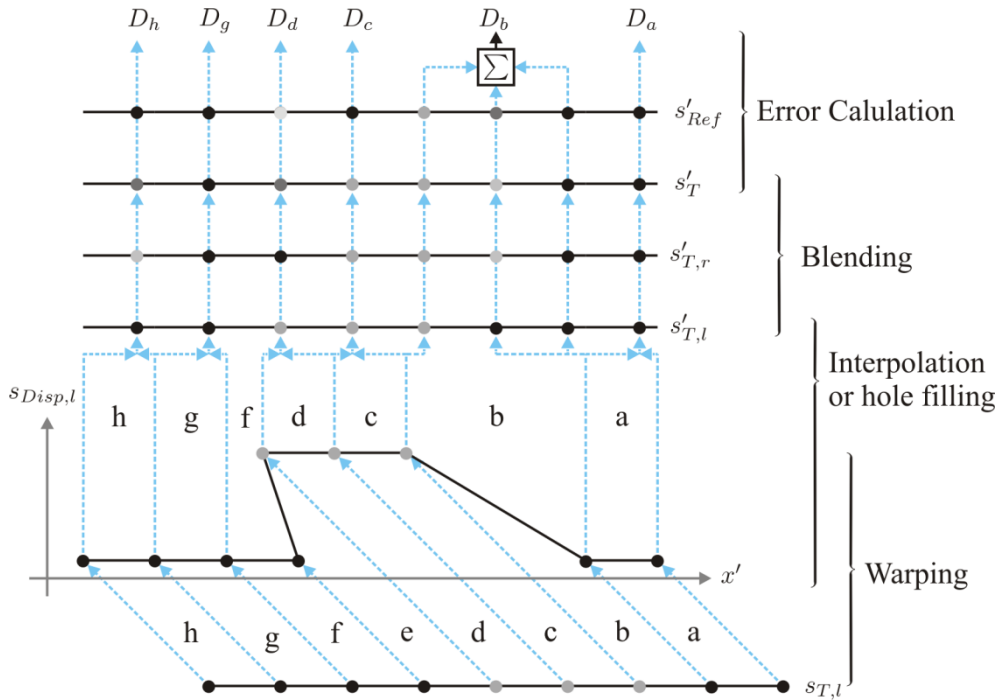
Figure 32: Example for the dependencies between input, intermediate and output signals of the rendering or error calculation step.
