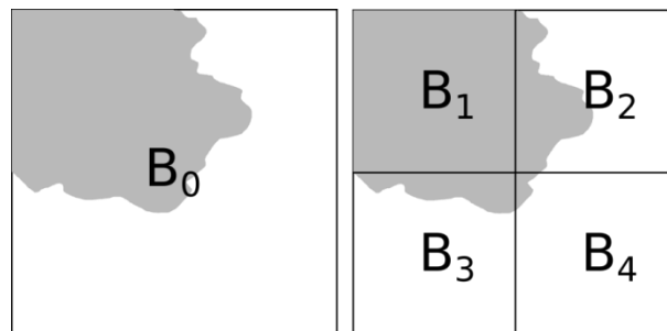
Figure 35: Distortion calculation on different tree depths. Renderable samples (gray shaded) are not taken into account.
