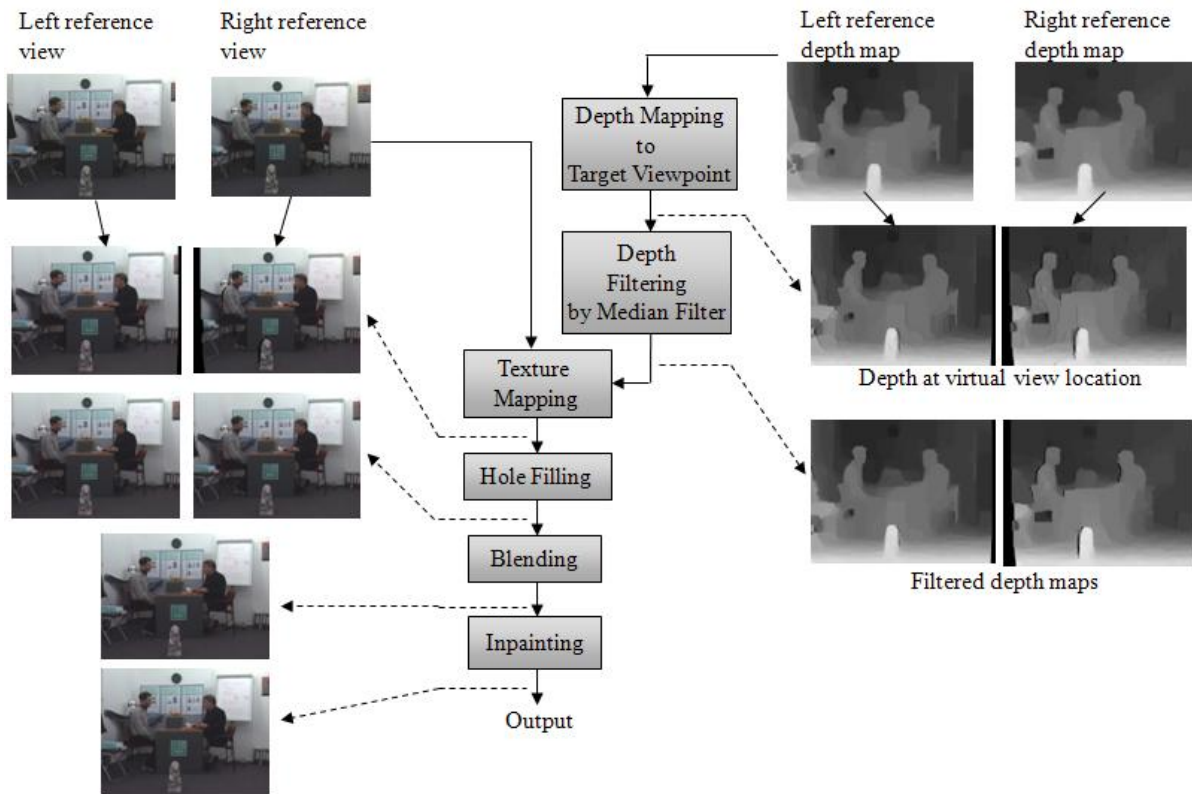
Figure 37: Flow diagram for VSRS general mode.
