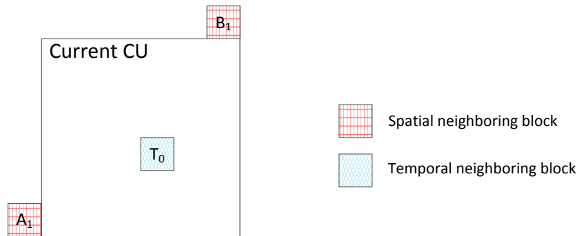
Figure 5: Location of spatial and temporal neighbour blocks
