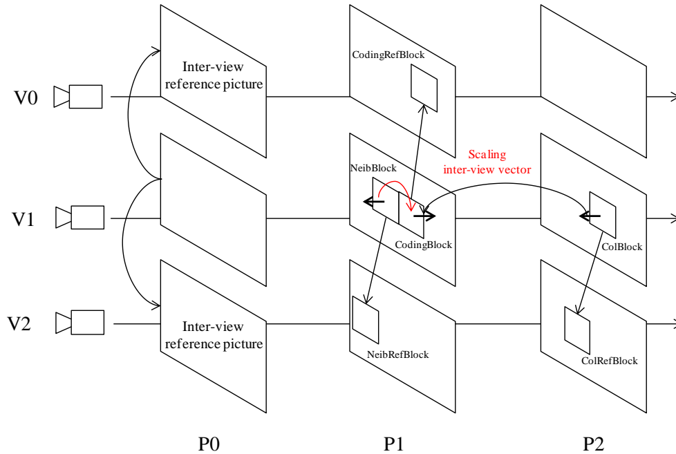
Figure 11: Inter-view motion vector scaling in TMVP
