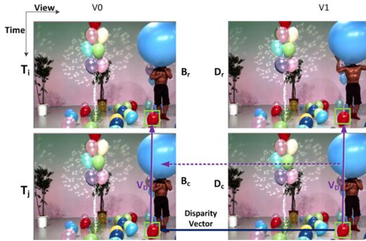
Figure 12: Prediction structure of the proposed ARP in 3D-HEVC.
