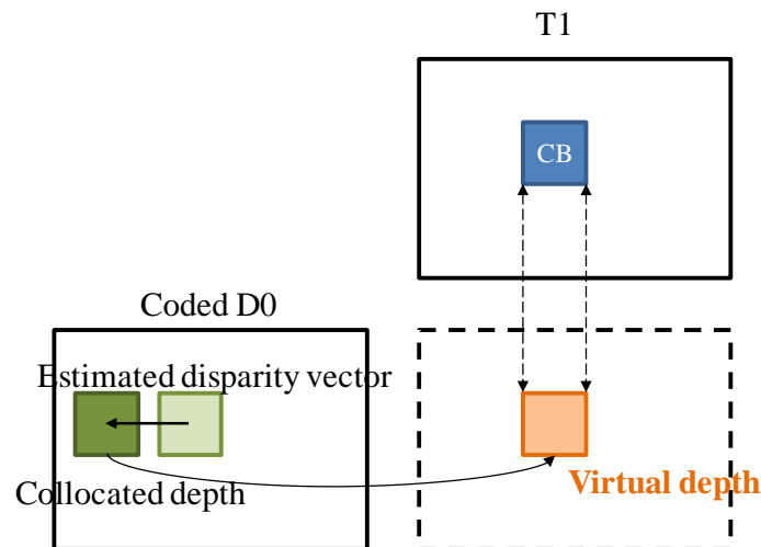
Figure 8: Retrieval of the virtual depth block.
