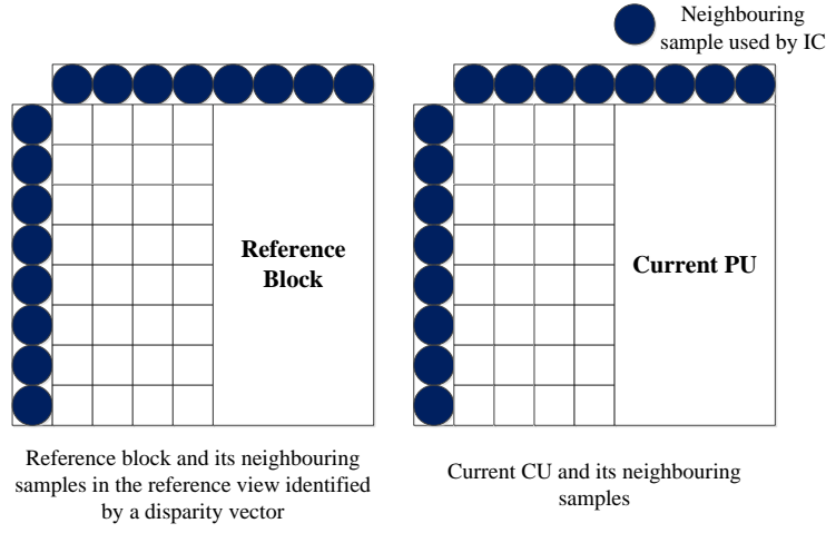
Figure 15: Neighbouring samples for the derivation of illumination compensation parameters.
