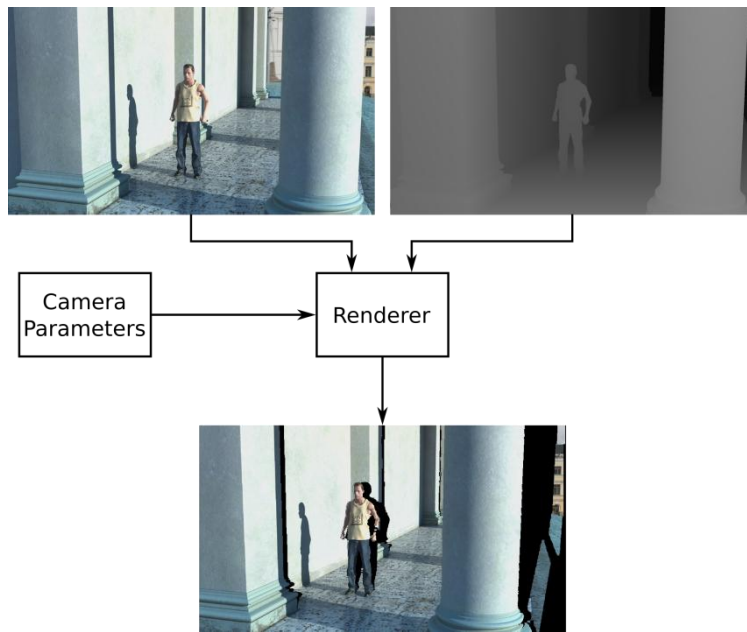
Figure 34: Rendering from a left camera position to a right camera position using depth maps.
