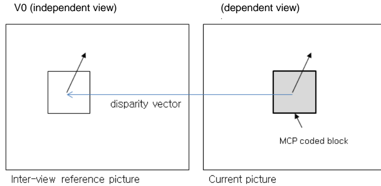
Figure 6: The inter-view predicted motion vector of a MCP coded block.
