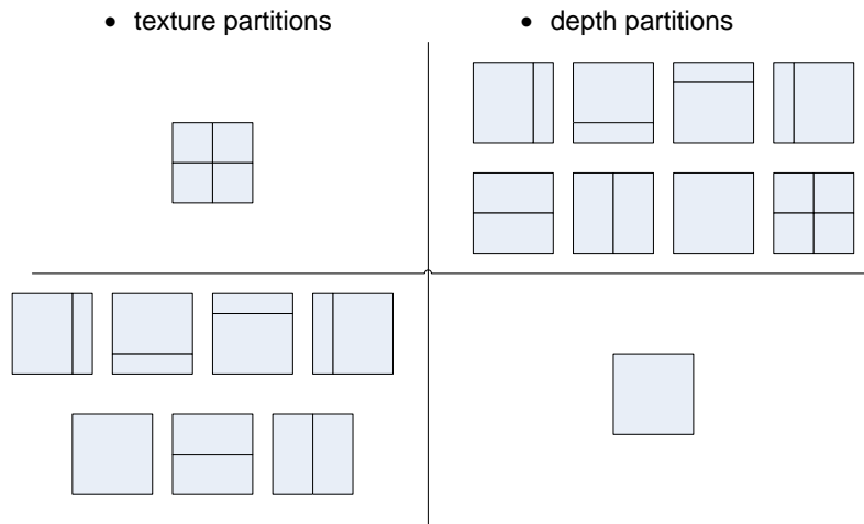
Figure 29: Texture partitions and corresponding possible depth partitions
