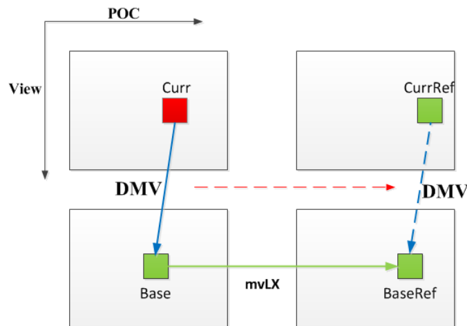
Figure 14. Prediction structure of ARP for inter-view residual.
