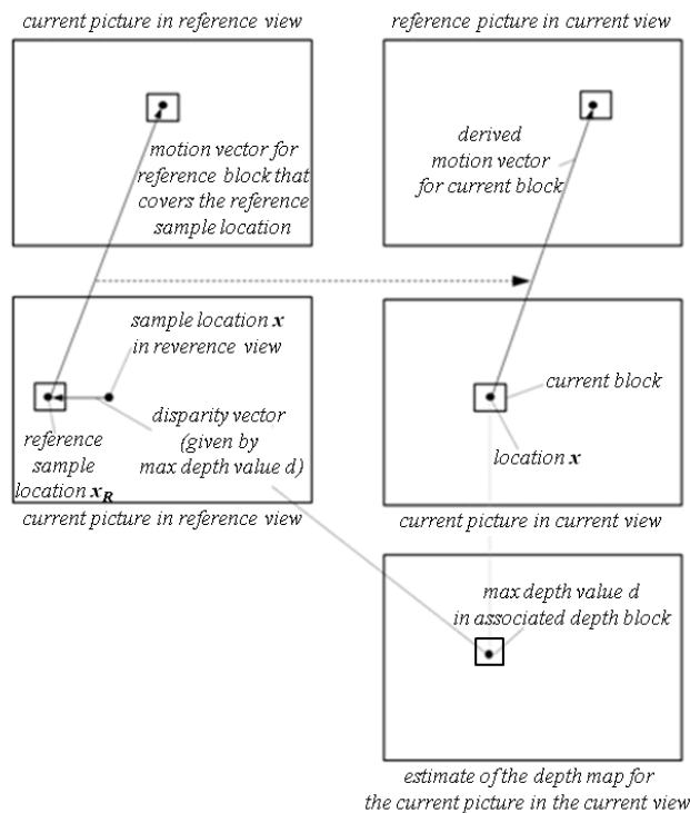
Figure 10: Basic principle of deriving motion parameters for a block in a current picture based on motion parameters in an already coded reference view and an estimate of the depth map for the current picture.
