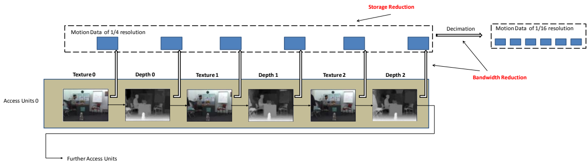
Figure 30: Progressive motion compression for motion data buffer reduction.
