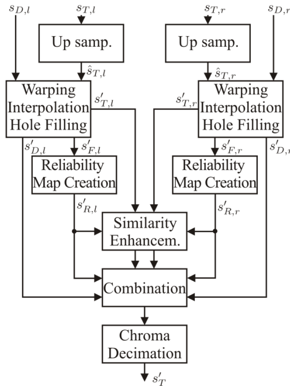
Figure 36: Processing steps of the view synthesis approach.
