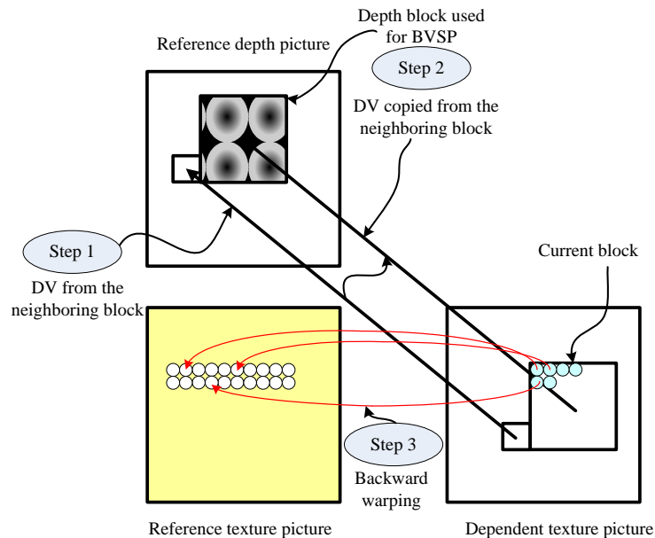
Figure 16: Illustration of the VSP scheme with the neighboring block disparity vector
