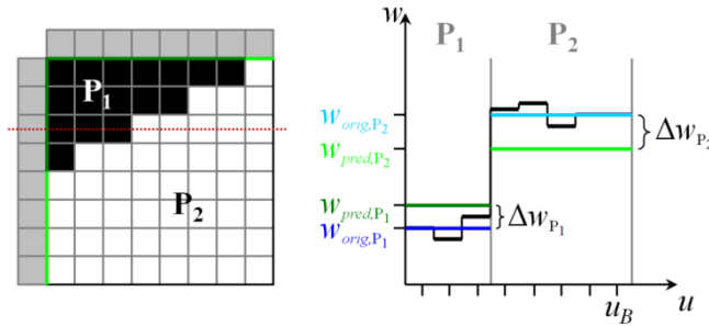
Figure 22: CPVs of block partitions: CPV prediction from adjacent samples of neighbouring blocks (left) and cross section of block (right), showing relation between different CPV types.
