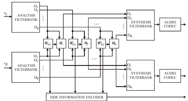
Fig. 1. General structure of the proposed matrix preprocessor
